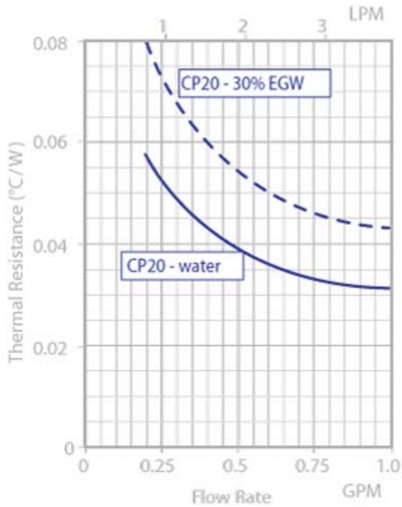
CP20 Thermal Resistance
