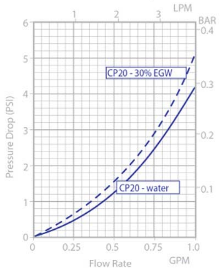
CP20 Pressure Drop
