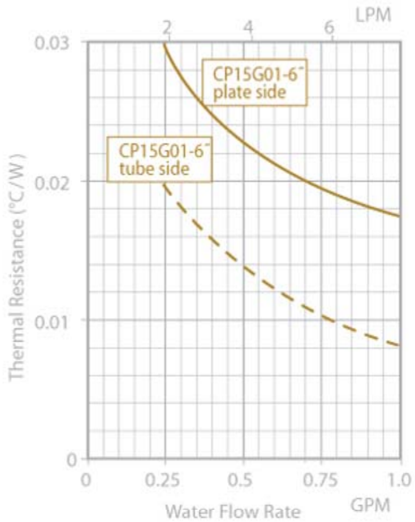
CP15G01 Thermal Resistance
