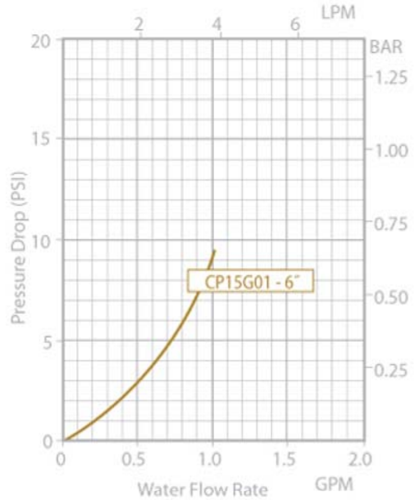
CP15G01 Pressure Drop
