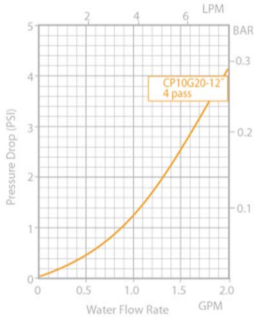
CP10G20 Pressure Drop
