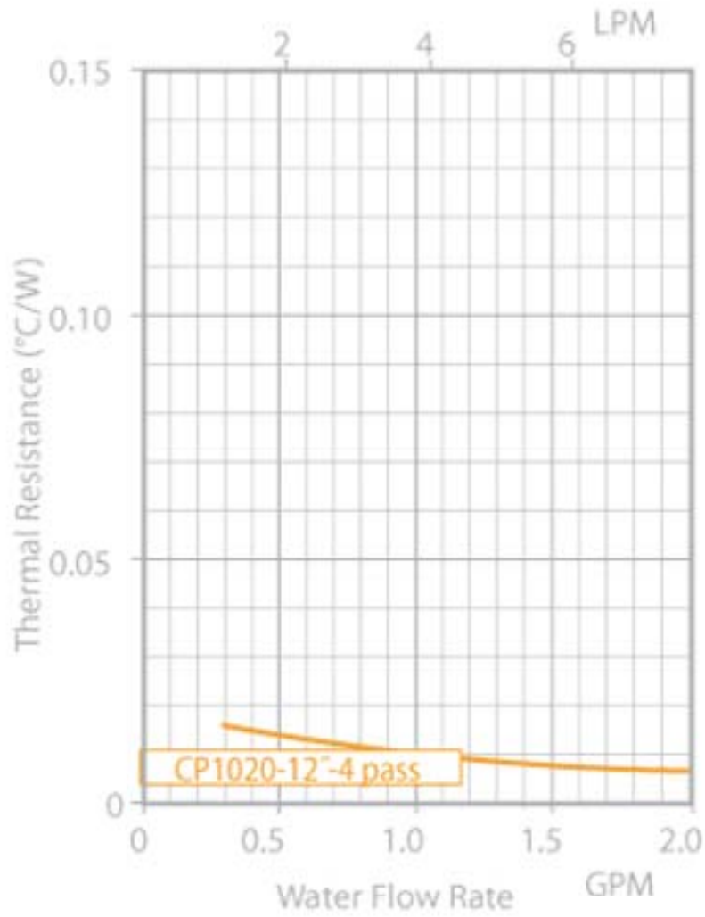
CP10G20 Thermal Resistance
