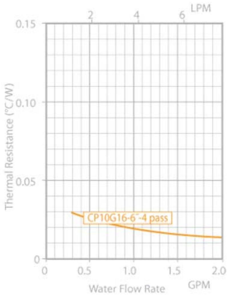
CP10G16 Thermal Resistance
