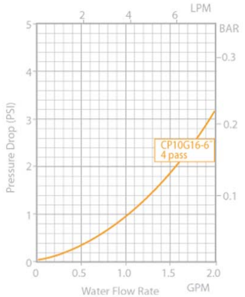
CP10G16 Pressure Drop
